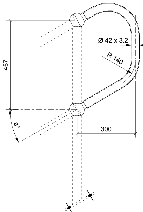
ACB-T (Angle Closure Bend -- Top)
